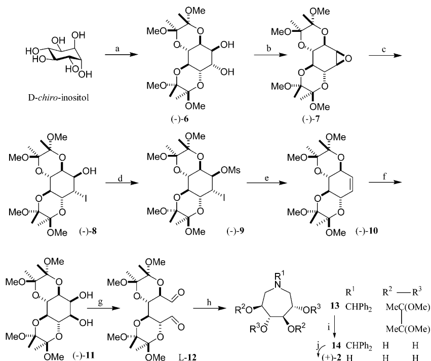
Scheme 1. Reagents and conditions: (a) butanedione, CH(OMe) 3 , H + , MeOH, reflux (80%); (b) Ph 3 P, DEAD, THF, 0 °C (68%); (c) AlCl 3 , MeCN, NaI, 0 °C (95%); (d) MsCl, Et 3 N, CH 2 Cl 2 (57%); (e) Zn dust, AcOH, DMF, 80 °C (92%); (f) NaIO 4 , RuCl 3 , EtOAc, MeCN, H 2 O (98%); (g) NaIO 4 , activated silica, CH 2 Cl 2 (90–95%); (h) NaCNBH 3 , MeOH, (Ph) 2 CHNH 2 , 3 Å sieves, 78 °C–rt; (i) TFA, H 2 O; (j) H 2 , Pd(OH) 2 /C, MeOH (h–j), 42%.
