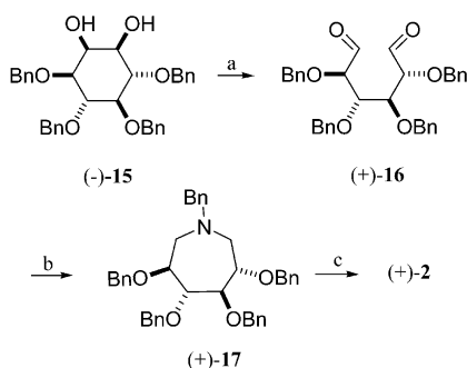
Scheme 3. (a) \text{NaIO}_4/\text{SiO}_2 , \text{CH}_2\text{Cl}_2 ; (b) \text{NaBH}(\text{OAc})_3 , \text{BnNH}_2 , \text{CH}_2\text{Cl}_2 , (a, b 86%); (c) \text{H}_2 , \text{Pd}(\text{OH})_2/\text{C} , \text{MeOH}/\text{AcOH} (trace) (92%).
