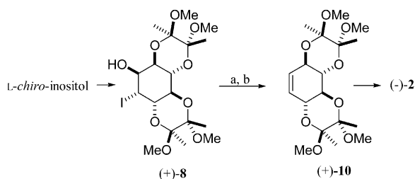
Scheme 2. (a) \text{TiF}_2\text{O} , Py, DMF; (b) Zn, AcOH (95%).
